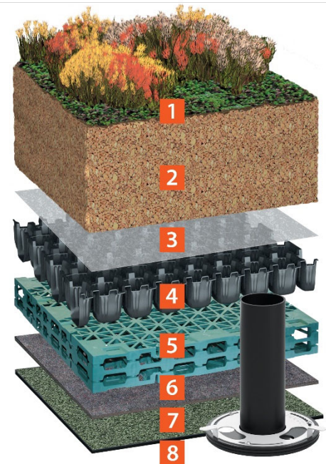
Indicative sedum blue roof system
