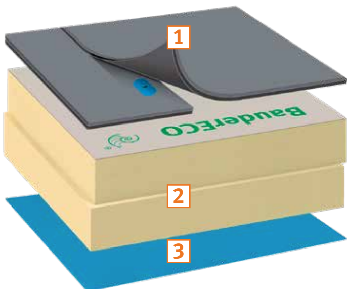
Mechanically fastened installation
