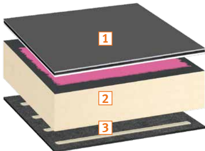
Adhered installation
